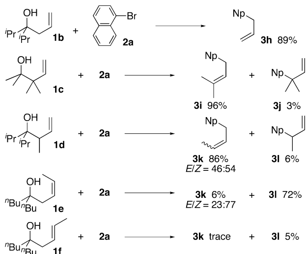
Scheme 2. Allylation of 2a with Various Homoallyl Alcohols a
