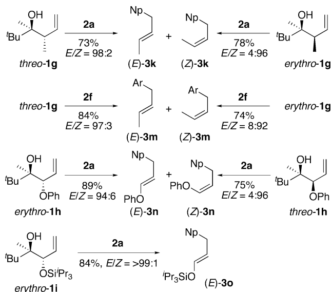
Scheme 3. Regio- and Stereospecific Allylation with Diastereomerically Pure Homoallyl Alcohols
